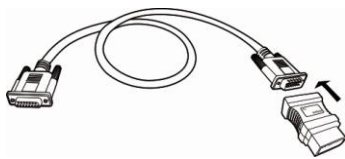
Figure 3.4: OBD I Adapter Connection to the DB15 Main Cable
